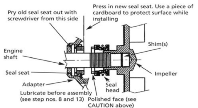
Figure 1B - Mechanical Seal Replacement
