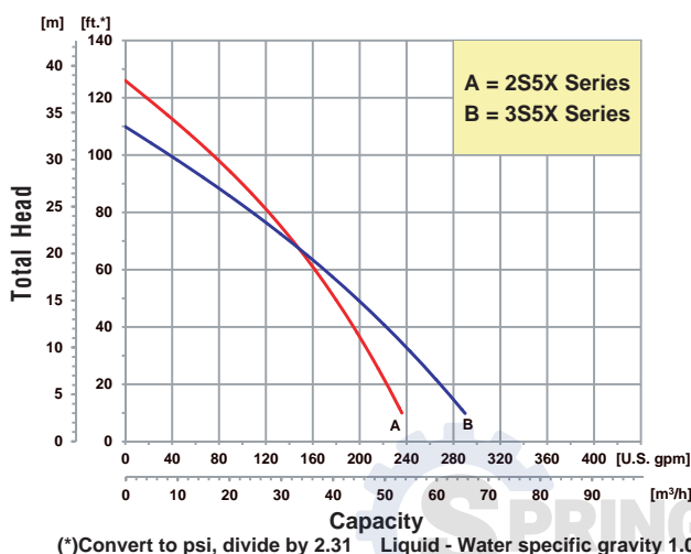
Performance of Engine Driven Self-Priming Trash Pumps
