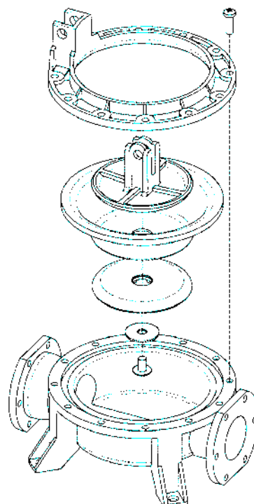
Figure 1 – Diaphragm Assembly
