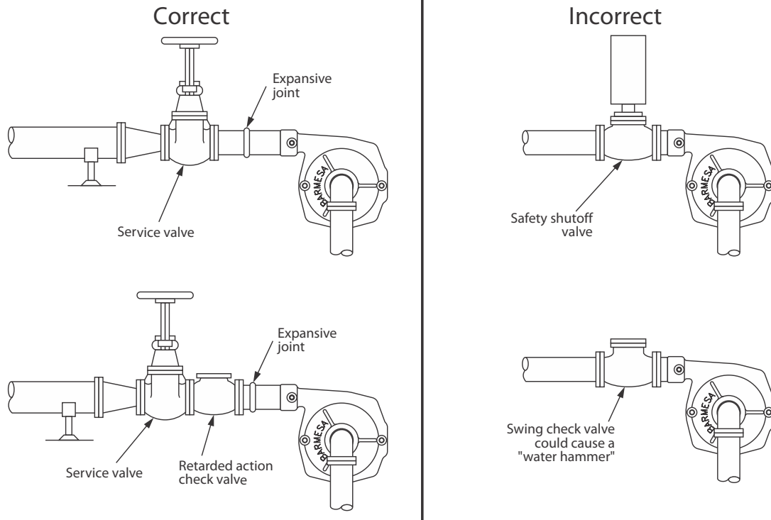
Figure 6 Discharge piping.
